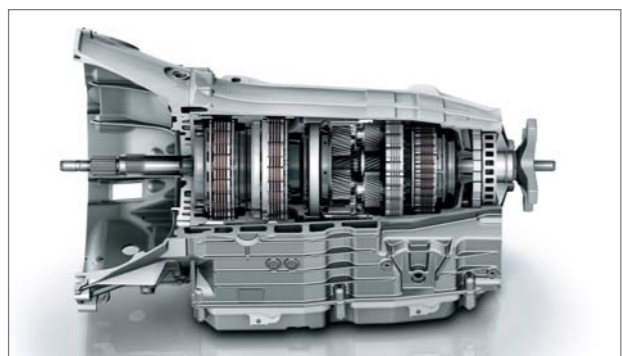
7G-TRONIC PLUS
