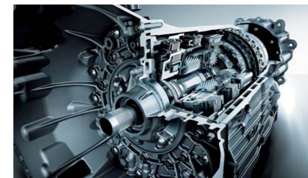
7G-TRONIC PLUS
