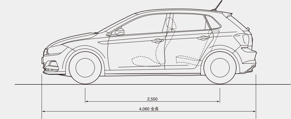
( )はTSI Highline
